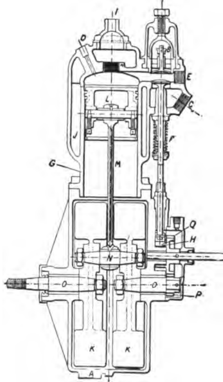
FIG. 382. —Section of the De Dion & Bouton Water-jacketed Carriage Motor, showing parts and construction of the engine shown in Fig. 380. The parts are as follows: A , the crank case formed by two cylindrical pieces bolted together; B is the inlet valve for the fuel mixture from the carburetter; C is the exhaust valve, formed of solid nickel steel, held closed by a helical spring, F , and opened at definite intervals by the cam, H ; D is the opening for screwing on the compression tap; E is the threaded hole for screwing in the sparking plug; F is the spring on the exhaust valve rod, which normally holds the valve closed; G is the cast iron cylinder which is bolted to the crank case; H is the exhaust cam cast in one piece with the gear, Q , which is actuated by the pinion, P , on the crank shaft; I is the port of exit for the jacket water circulating through the jacket, J , the inlet being at a point near the base of the jacket; K and K are the fly-wheels, or crank-discs, which are joined together as shown, by the crank pin, N ; L is the piston whose construction corresponds to that shown in Fig. 284; M is the connecting rod of drop-forged steel; N is the crank or wrist pin connected to the fly-wheel as shown, and serving as a bearing to the lower end of the crank rod; O and O are the crank shafts, that on the right carrying the pinion, P , that on the left being threaded for connection to the driving gear; P is a pinion on the crank shaft meshing with gear, Q , on the cam shaft.
